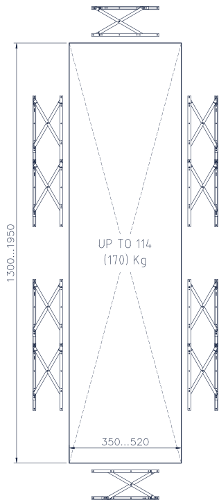
2x(KFS-PH-CP-12)+4x(KFS-PH-CP-24) UP TO 114 Kg 2x(KFS-PH-12)+4x(KFS-PH-24) UP TO 170 Kg
