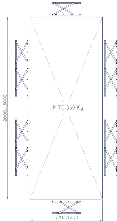
2x(KFS-PH-18)+4x(KFS-PH-36) UP TO 360 Kg
