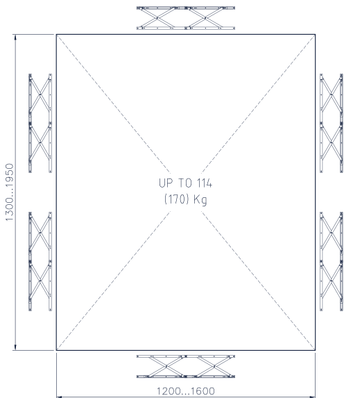
6x(KFS-PH-CP-24) UP TO 114 Kg 6x(KFS-PH-24) UP TO 170 Kg
