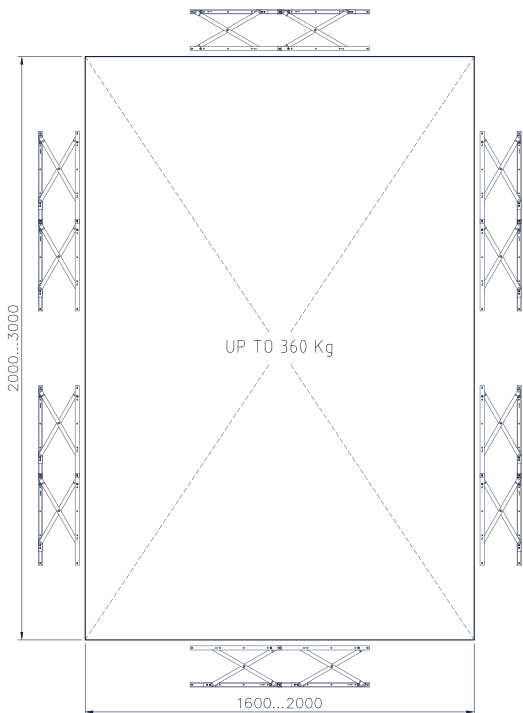
6x(KFS-PH-36) UP TO 360 Kg
